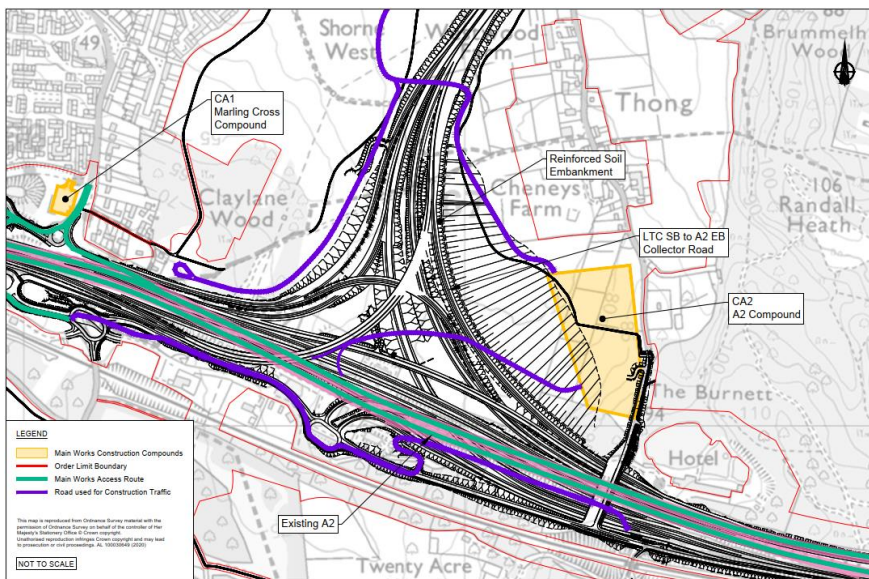
Plate 7.6 Location of reinforced soil embankment
